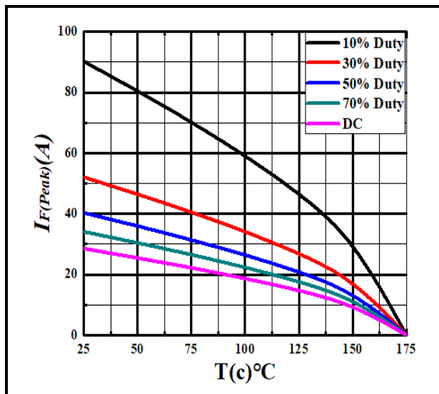
Figure 3. Current Derating
