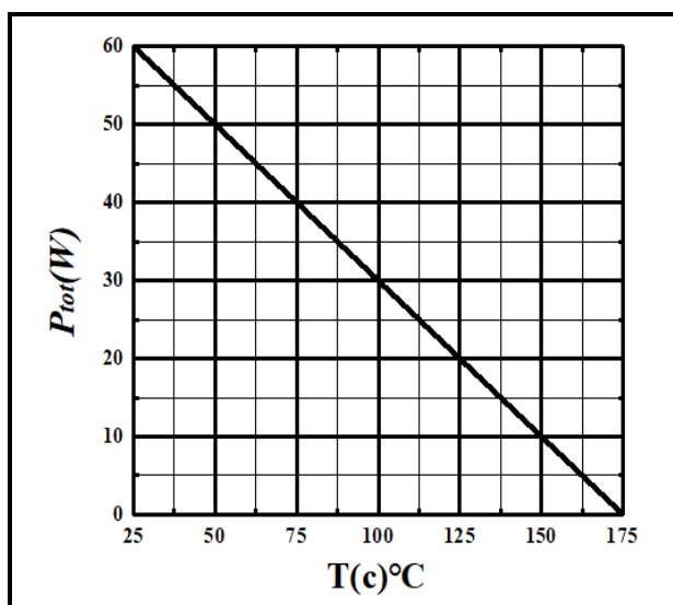
Figure 5. Power Derating
